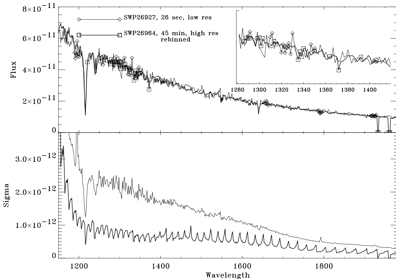
Fig. 7. Comparison of low resolution (thin line) and high resolution rebinned (thick line) spectra of the standard star BD+28 4211. The top panel shows the flux spectra. Flagged pixels are marked with diamonds (low resolution) and squares (rebinned). The two gaps in the high resolution spectra longward 1900 Å correspond to the regions where spectral orders do not overlap, which have been assigned zero flux. The inset in the top panel shows in more detail the region 1300–1400Å. The error spectrum is shown in the bottom panel (thin line: low resolution, thick line: rebinned). The characteristic pattern of the errors of the rebinned spectrum is due to the lower signal-to-noise ratio at the edges of the individual echelle orders.
