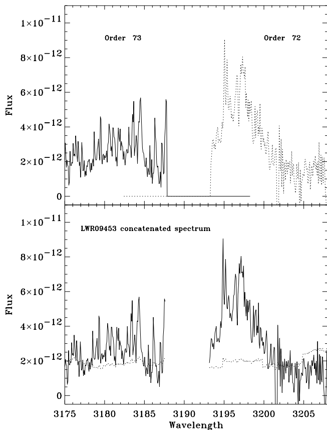
Fig. 6. As Figure 4 for the LWR camera. In the spectral region shown orders do not overlap. The INES concatenated spectrum has no data in that region.
