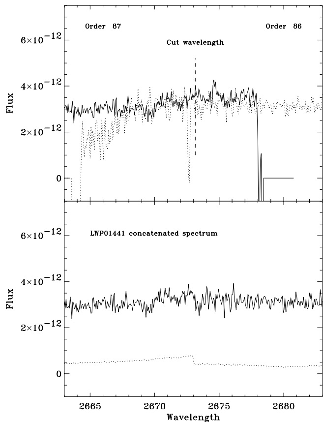
Fig. 5. As figure 4 for the LWP camera.
