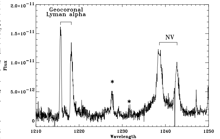
Fig. 1. A portion of the longest available SWP exposure of RR Tel (SWP20246: 820 minutes). The two Lyman \alpha lines arise from geocoronal emission filling the large and the small apertures. The emission features labeled with an asterisk are due to overspilling of the strong NV emission into the adjacent order.
