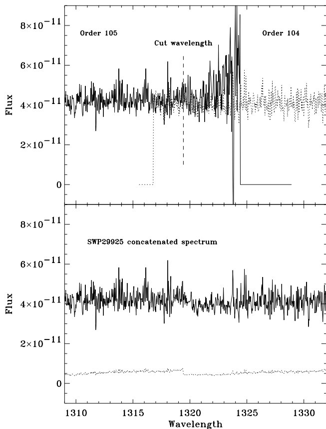
Fig. 4. Example of the concatenation procedure for the SWP camera. The top panel shows the individual orders from the MXHI file. The bottom panel shows the final concatenated spectrum and the calibrated errors (dotted line).
