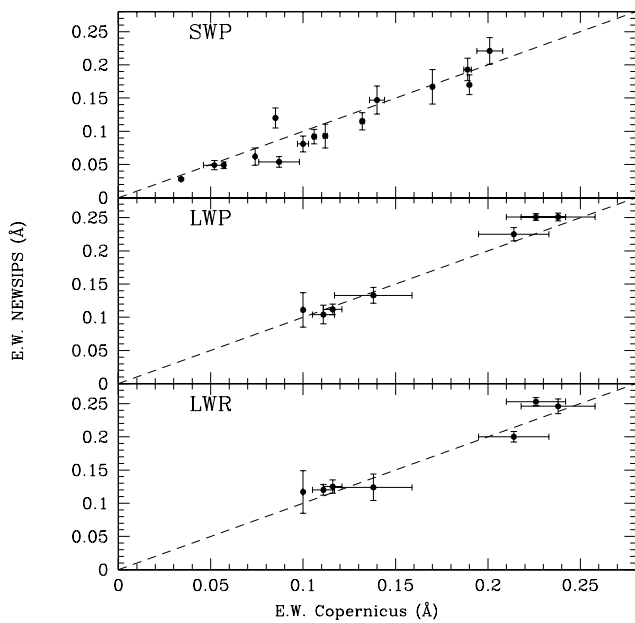
Fig. 2. Comparison of the equivalent widths of interstellar lines in the spectrum of \zeta Oph as measured in Copernicus and in NEWSIPS spectra. Copernicus measurements have been taken from Morton (1975). The dashed line in each panel indicates the 1:1 relation.
