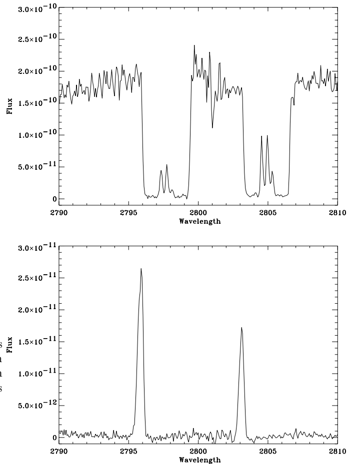
Fig. 3. Top panel: The region of the MgII doublet in the spectrum of SN 1987A (LWP10194). Bottom panel: The same region in the deepest LWP exposure of RR Tel (LWP25954).
