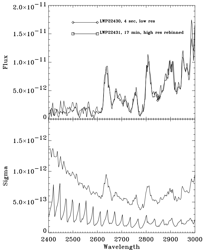
Fig. 8. Similar to Figure 7 but comparing two LWP spectra of Nova Cygni 1992. The errors are shown in the bottom panel.
